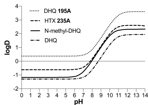
FIGURE 2 Predicted logD of decahydroquinoline (DHQ), N-methyl decahydroquinoline (N-methyl-DHQ), decahydroquinoline 195A (DHQ 195A ), and histrionicotoxin 235A (HTX 235A ) ranging from 0 to 14 pH
