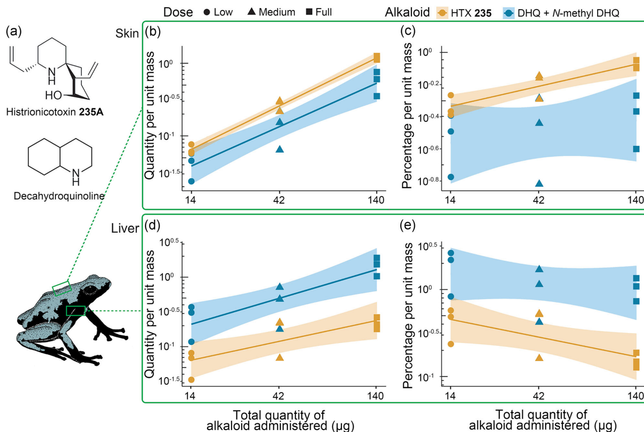
FIGURE 1 Dose response and efficiency of accumulation of histrionicotoxin (HTX) 235A and decahydroquinoline (DHQ + N-methyl DHQ). (a) Chemical structures of HTX 235A and DHQ used in the experiments. Dose response accumulation of both alkaloids in (b) skin and (d) liver. Accumulation efficiency of both alkaloids in (c) skin and (e) liver. Each symbol represents an individual of Adelphobates galactonotus for each experimental group ( n = 3 ). Quantity and percentage of alkaloid detected per unit mass were \log_{10} transformed for the simple regression. Regression lines are only included for results that were statistically significant
